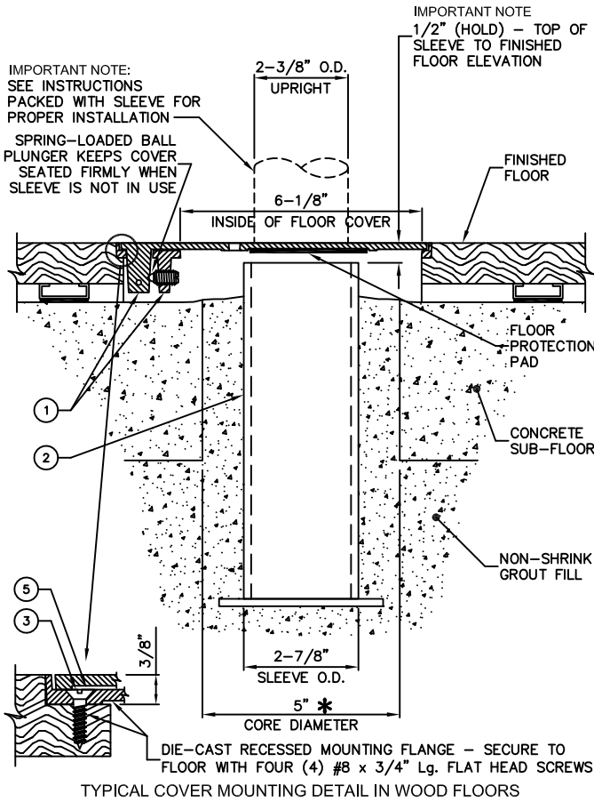
TYPICAL COVER MOUNTING DETAIL IN WOOD FLOORS
