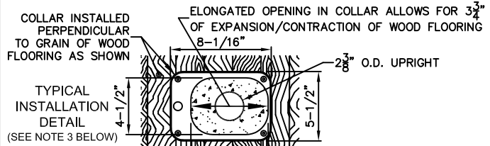
TYPICAL INSTALLATION DETAIL (SEE NOTE 3 BELOW)
