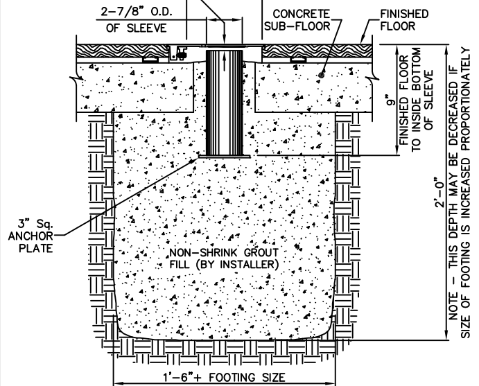
INSTALLATION OPTIONS (COMPLETE INSTALLATION INSTRUCTIONS ARE INCLUDED WITH FLOOR SLEEVE.)
